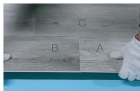
❸ Uplift the A and B flooring at the same time (Note: the two flooring need in same direction and 45 degree with ground)
