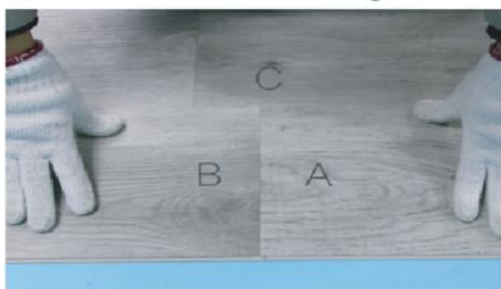
❹ Put the A floor flat, It can be adjusted by tapping gently so that there are no gaps between the floors
